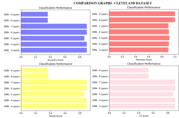
Fig 4: Comparison of DNN Layers with Cleveland Dataset
