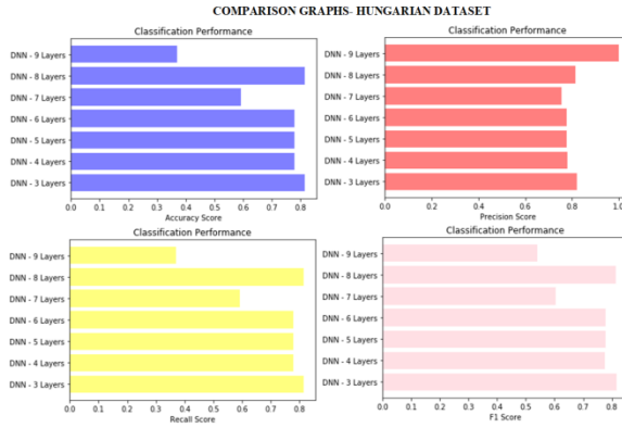
Fig 6: Comparison of DNN layers with Hungarian Dataset
