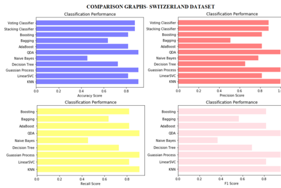
Fig 7: Comparison of All Algorithms with Switzerland Dataset
