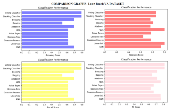
Fig 9: Comparison of All Algorithms with Long Brach VA Dataset
